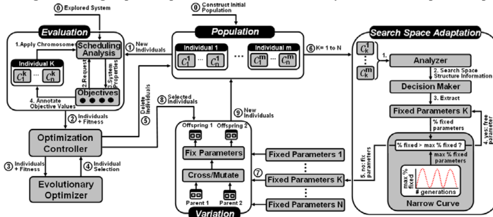
Figure 1. Design Space Exploration Framework with Dynamic Search Space Adaptation
