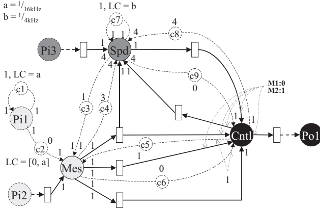
Figure 9. SPI representation of the controller
