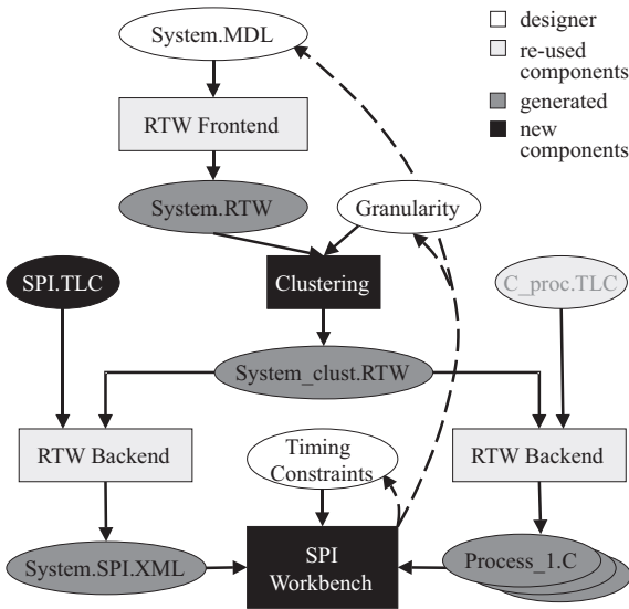
Figure 7. Design flow
