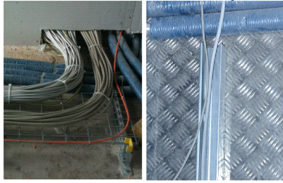
Figure 3. Wirings looms and single wire
