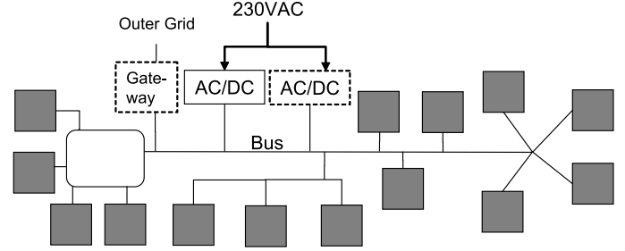
Figure 1. SmallCAN System
